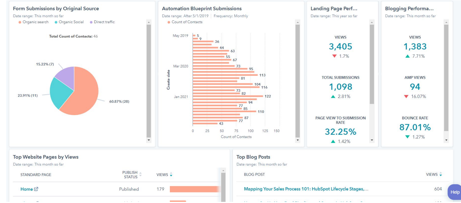
HubSpot Example
