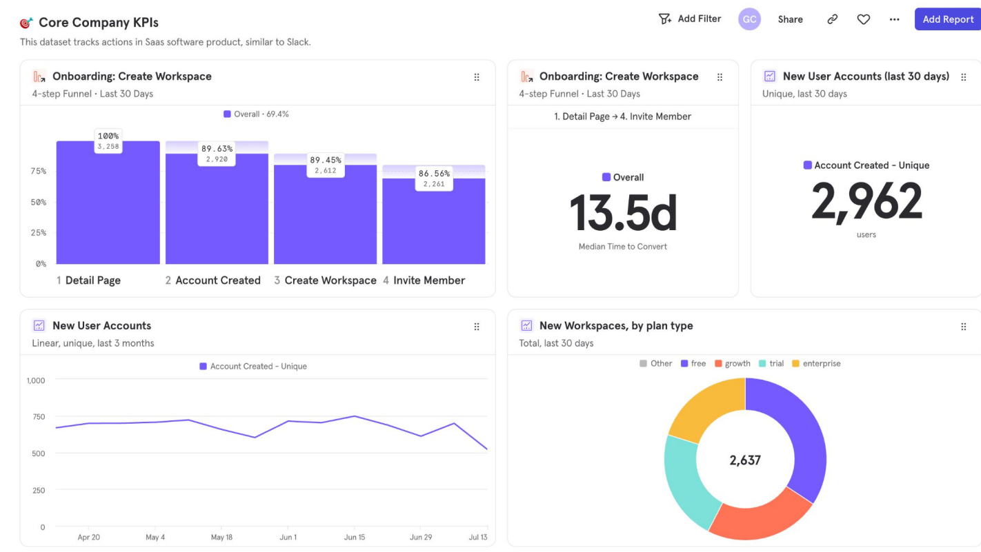
Mixpanel Example
